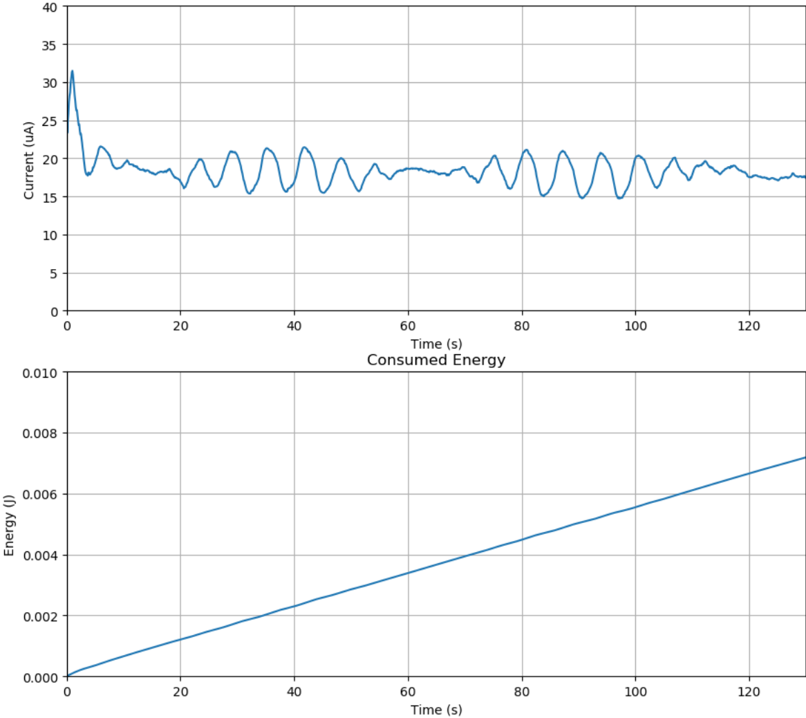
Aurora XLDSN3 NBloT Variant Sleep Current, no sensor board. dT = 100.0000 ms
