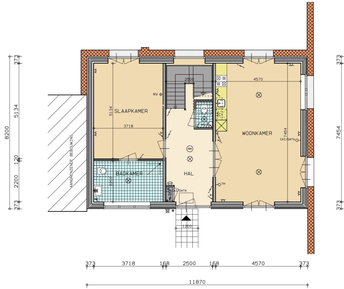
BEGANE GROND > BOUWNR. 3 (TYPE: D) VARIANT 2 BADKAMER
