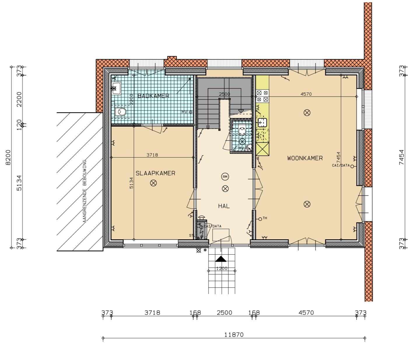
BEGANE GROND > BOUWNR. 3 (TYPE: D) VARIANT 1 BADKAMER
