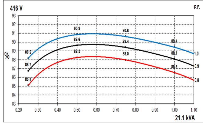
60Hz Curves
