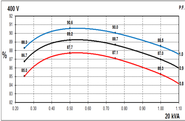
50Hz Curves
