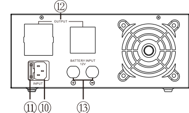
Back panel
