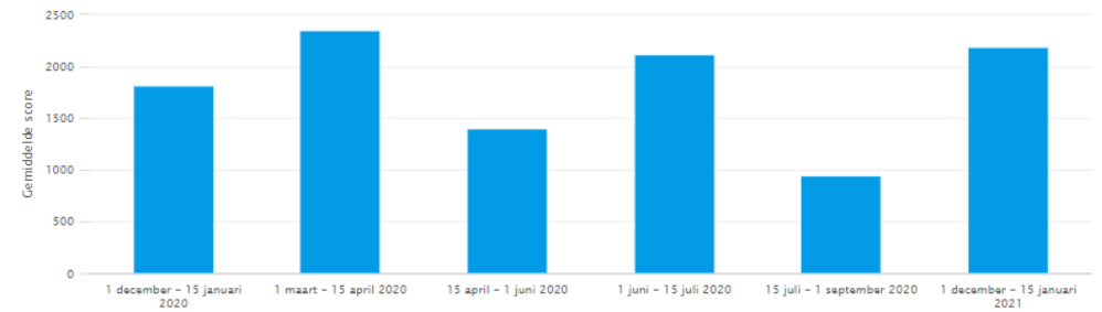
Challenge scores
