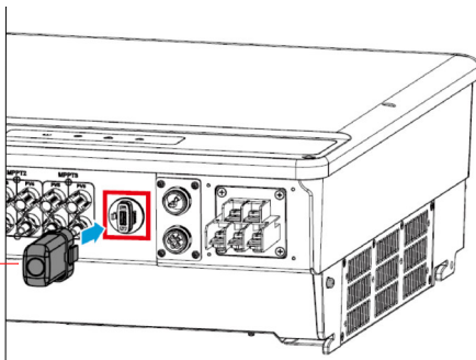
Communication module
