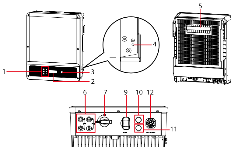
Viessmann PV Inverter 4D-3, Viessmann PV Inverter 5D-3, Viessmann PV Inverter 6D-3
