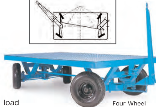
Four Wheel Steering Ackerman Trailer
