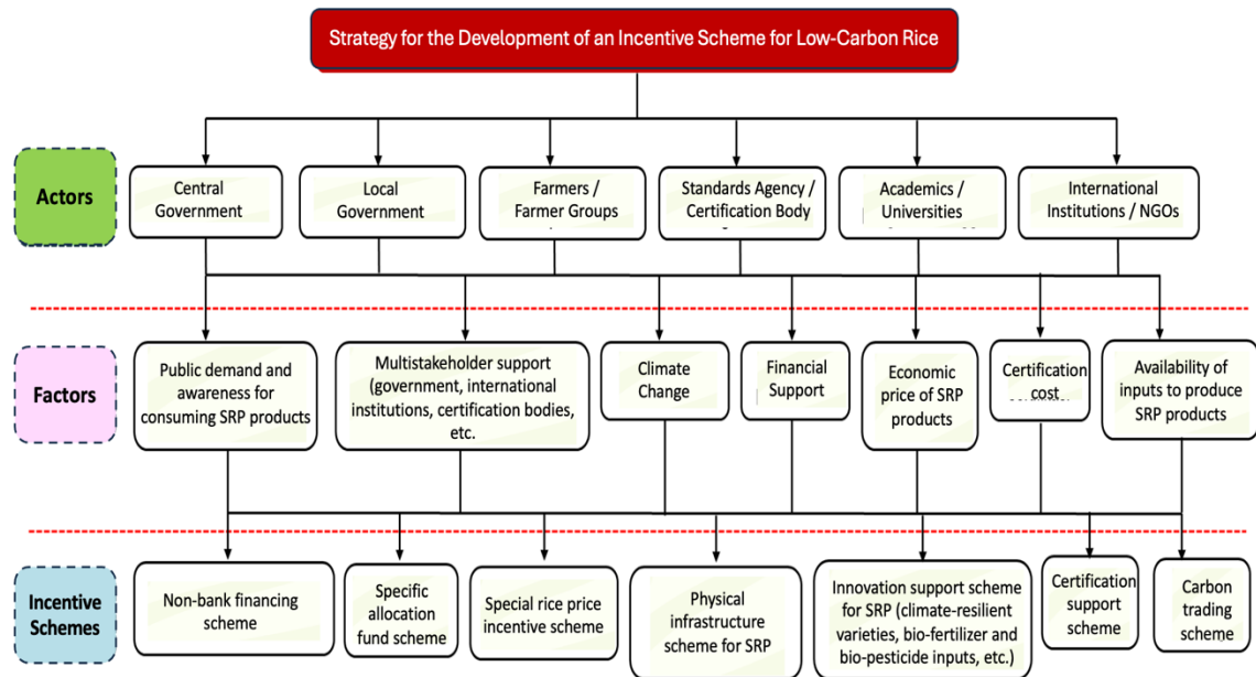
Figure 6. Analytical Hierarchy Process (AHP) Hierarchy Tree
