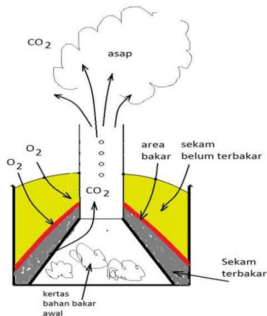
Figure 6, Mechanism of husk charcoal formation
