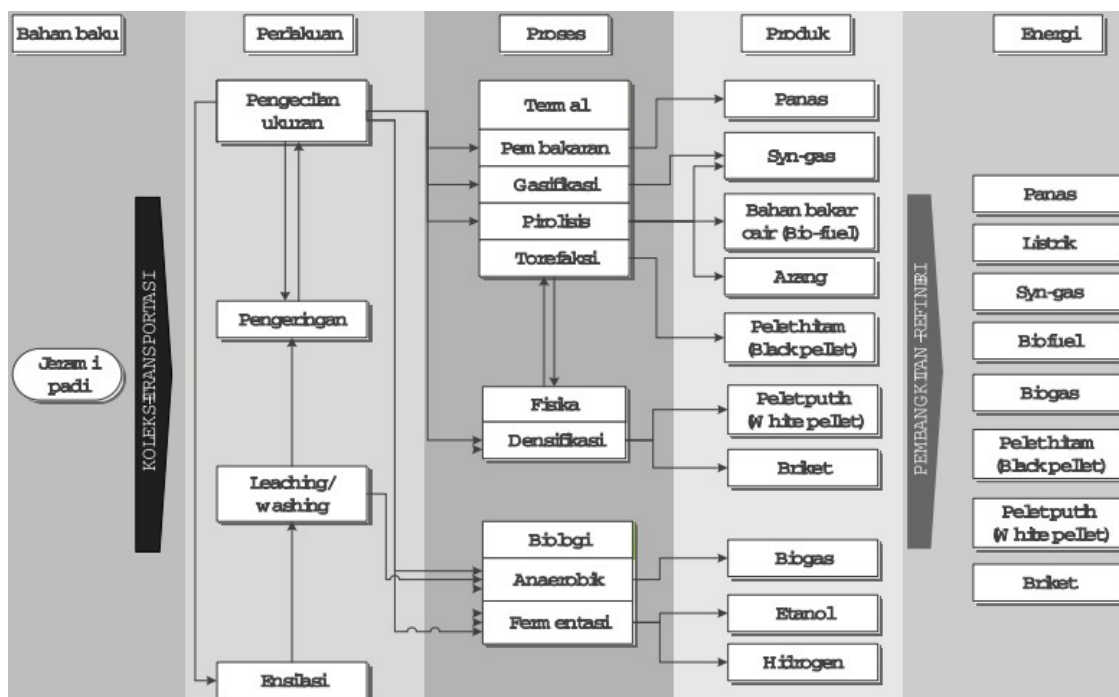
Potential Rice Straw Energy Conversion Process (IRRI, 2018)
