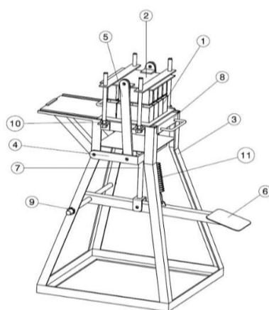
Figure 8. Husk charcoal briquette moulding machine
