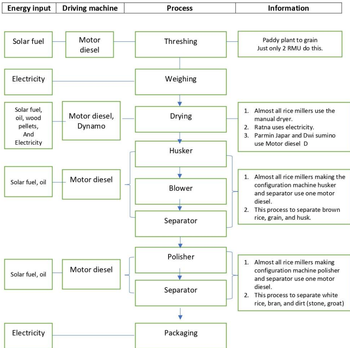
Figure 3: Production process map
