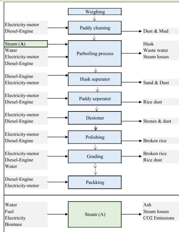
Figure 2: Process flow diagram of rice mills
