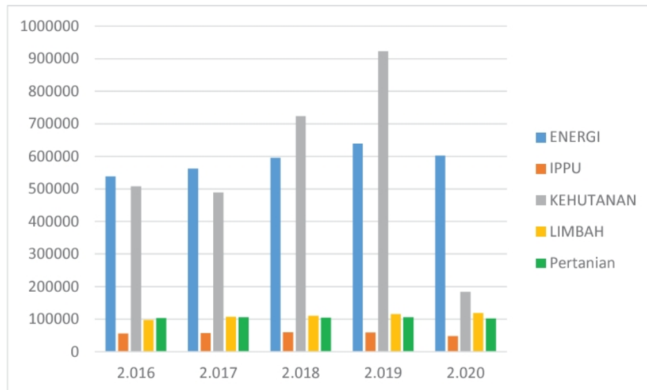
GHG EMISSIONS (Gg CO 2 ) from 2016-2020 (Balington, 2021)
