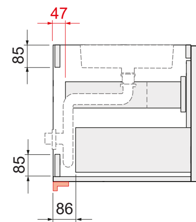
side - section
