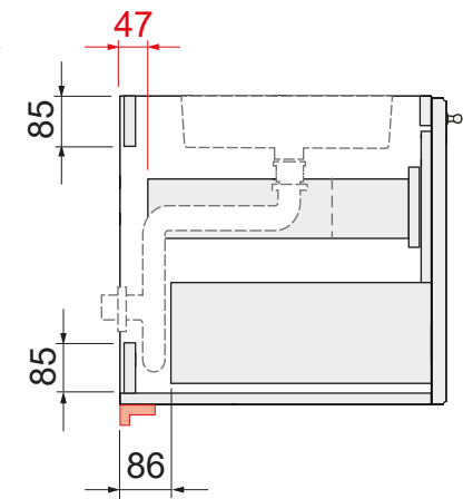
side - section
