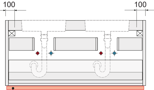
front - section
