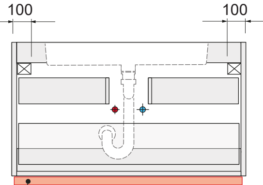
front - section
